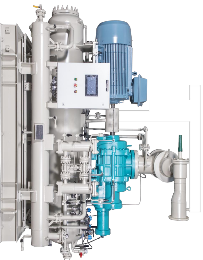
KRS - SCREW PACKAGE
