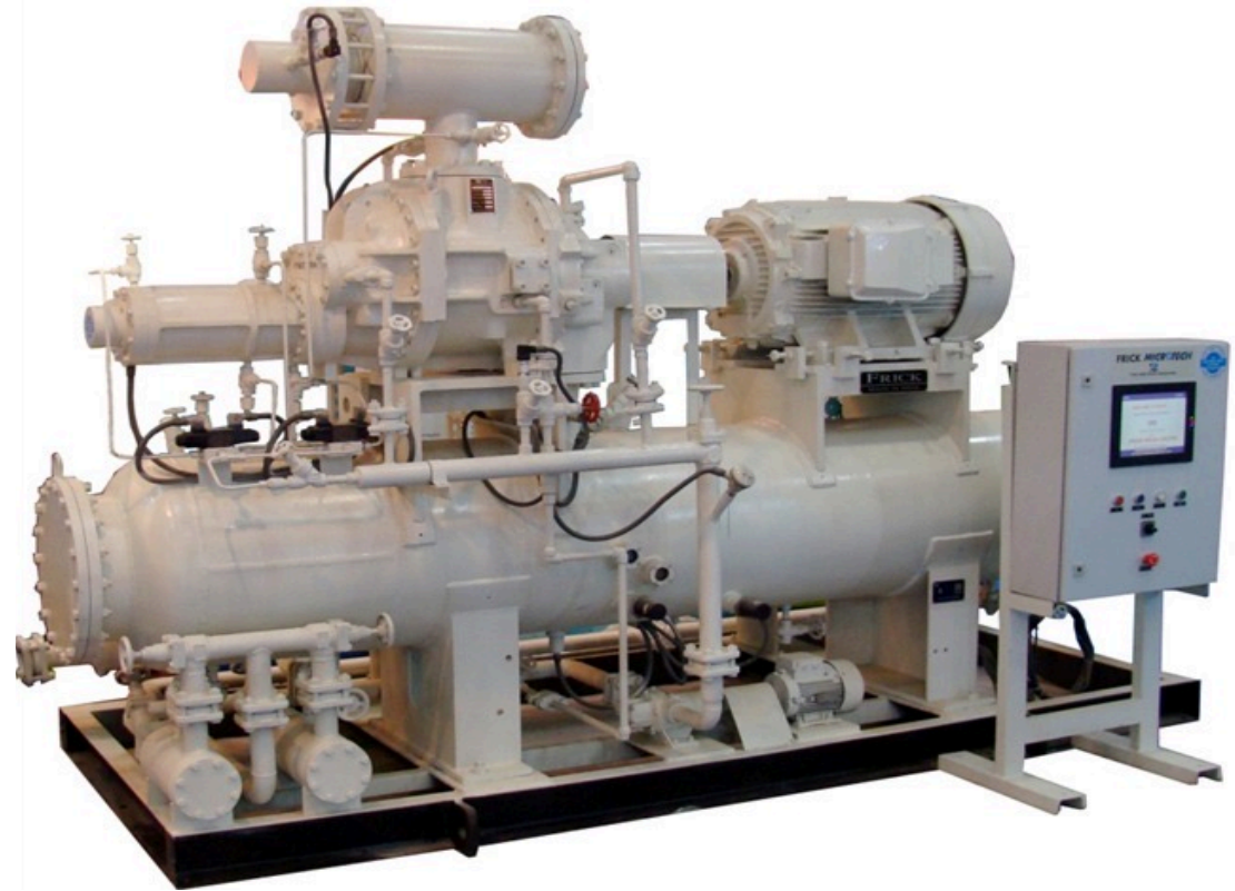
Frick India Screw Package (with Frick Screw Block)
